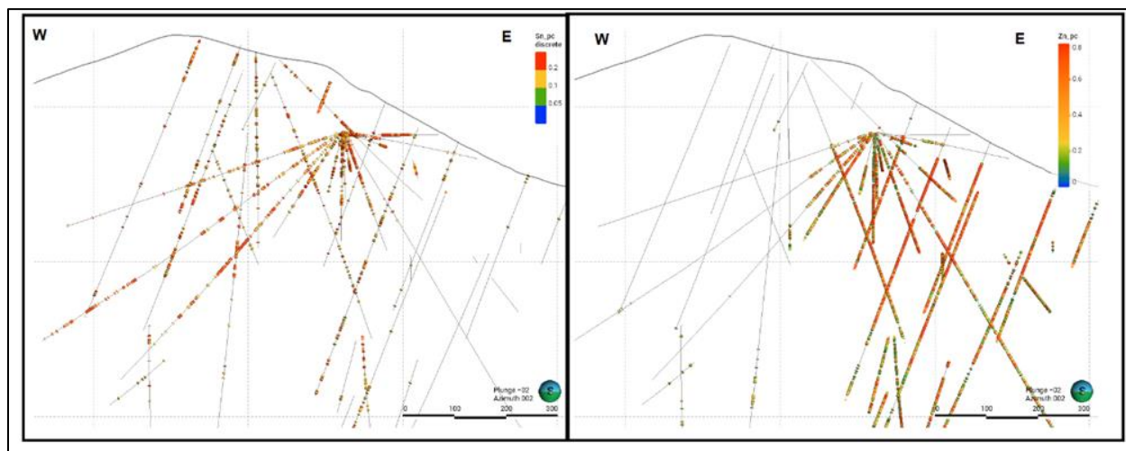
Figure 25.3 Section Through the Iska Iska Deposit Showing the Distribution of Sn > 0.1% and Zn > 0.5%, respectively.
