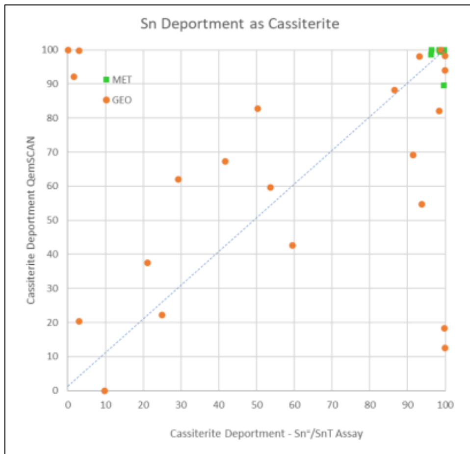
Figure 3 Tin deportment as cassiterite based on geochemistry and mineralogy. Only samples >0.1% Sn (T).
