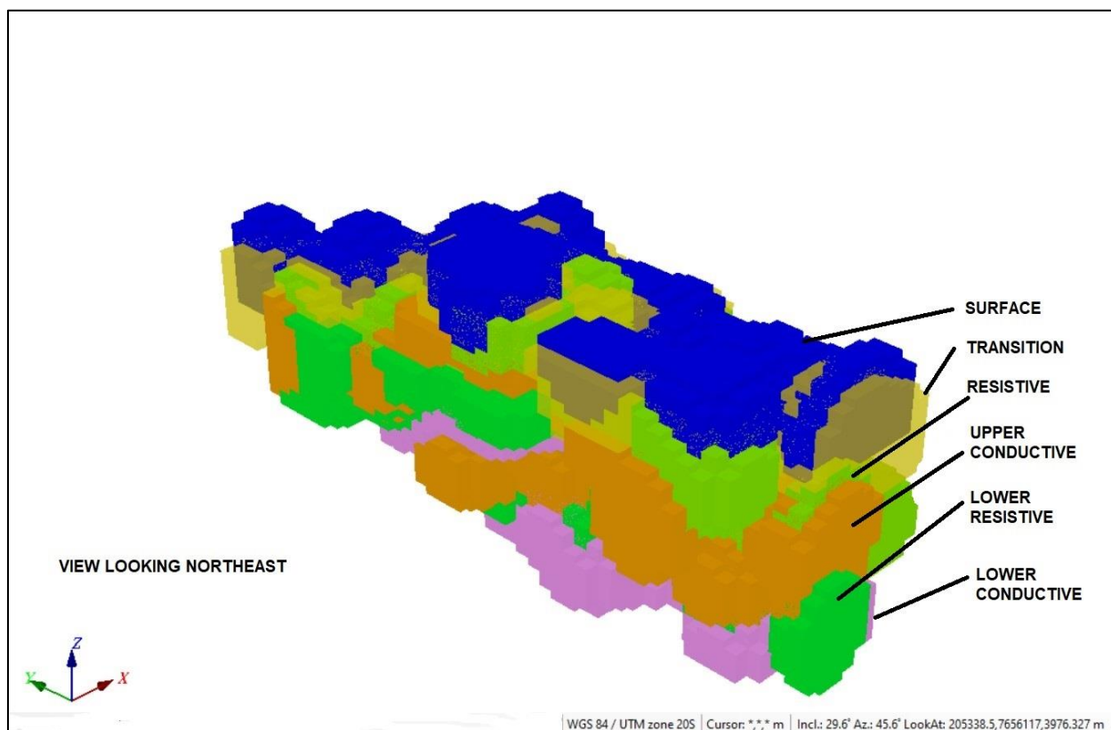
Figure 9.10 Lithological Domains suggested by BHIP Conductivity Data
