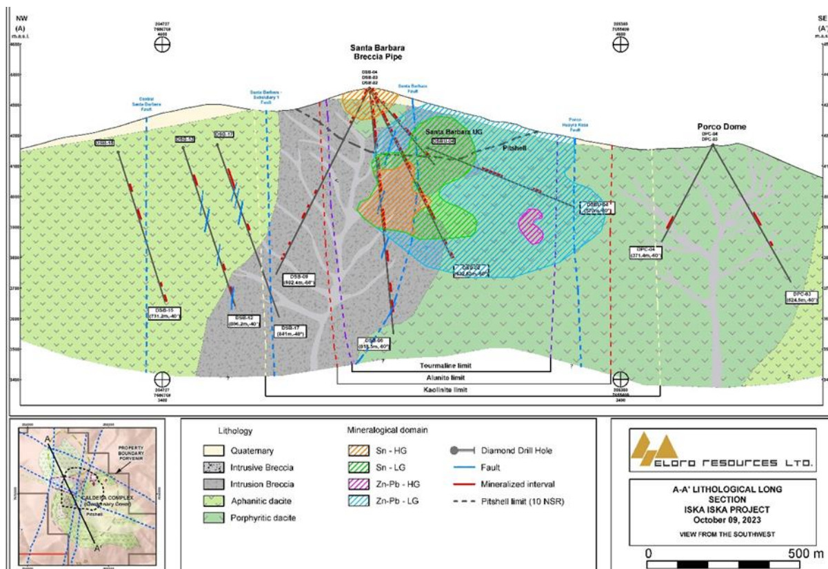
Figure 7.8 Longitudinal Geological Section Showing Distribution of Major Lithologies at Iska Iska
