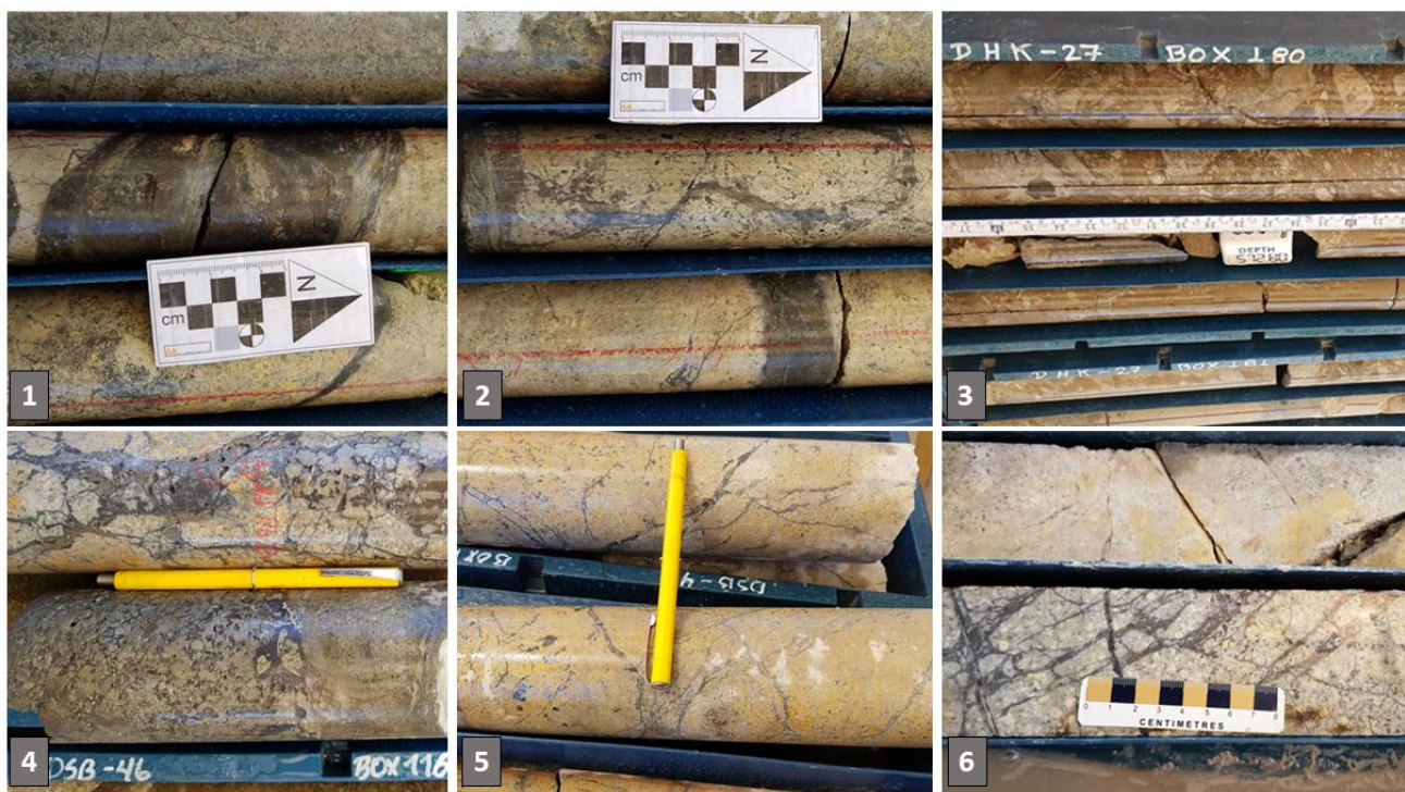
Figure 12.3 Mineralization Styles/Patterns Observed at Iska Iska
