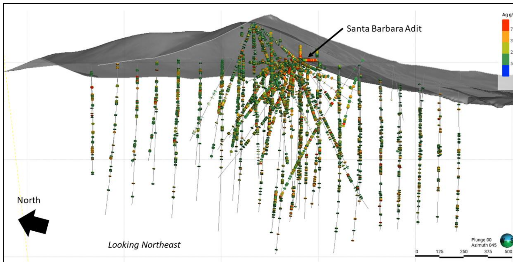
Figure 1.3 Vertical Section Through the Iska Iska Deposit Showing Ag Assays > 10 g/t in Drillholes.
