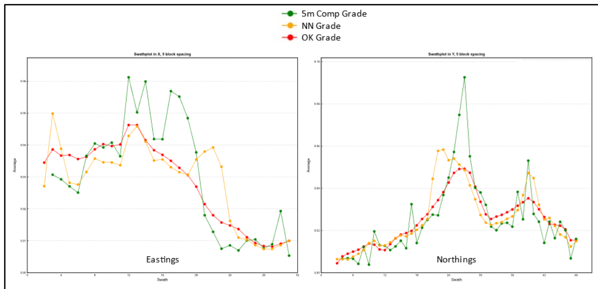
Figure 14.21 Iska Iska 50 m Swath Plot for Sn in MinZone 30
